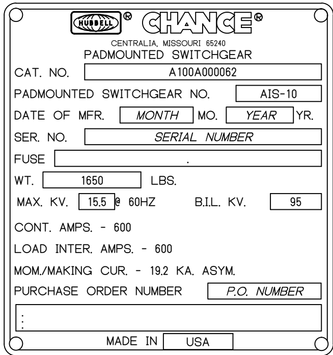
NAMEPLATE DETAIL (4X)
