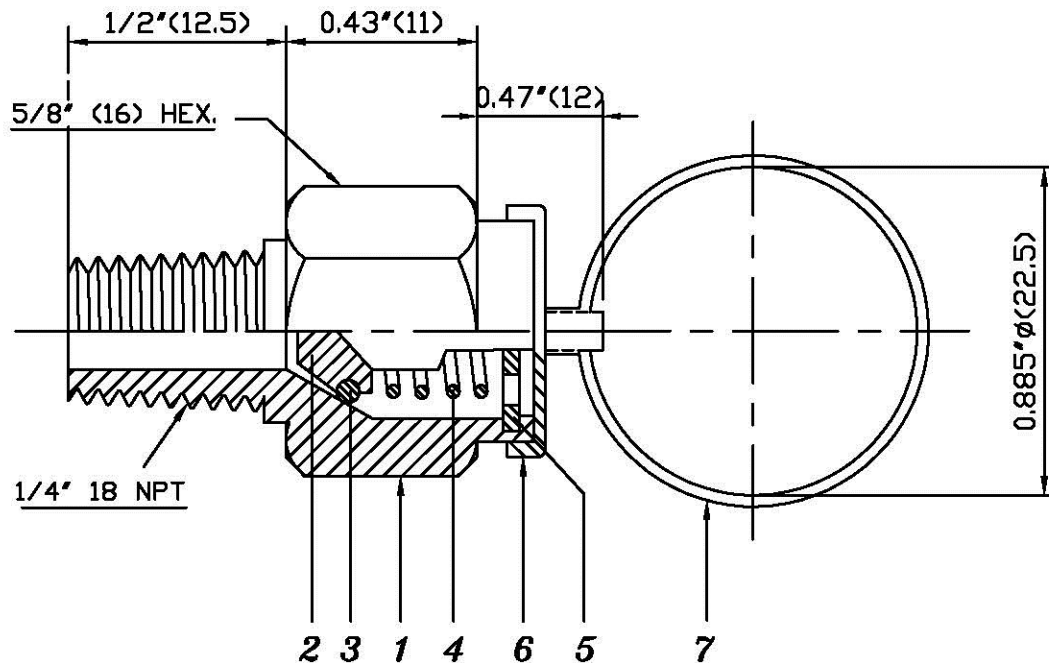
SECTIONAL FRONT VIEW
